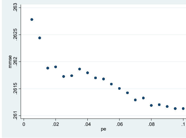
Average MSE
